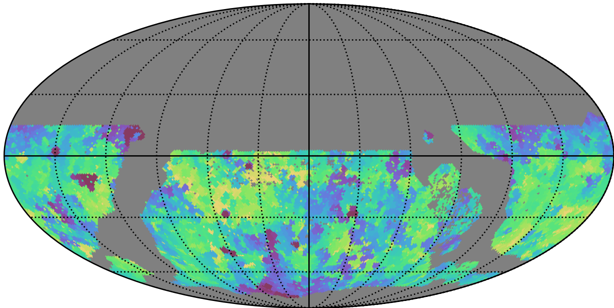
ddf_loaded_fl15_v3.4_10yrs WFD g band: Min fiveSigmaDepth
