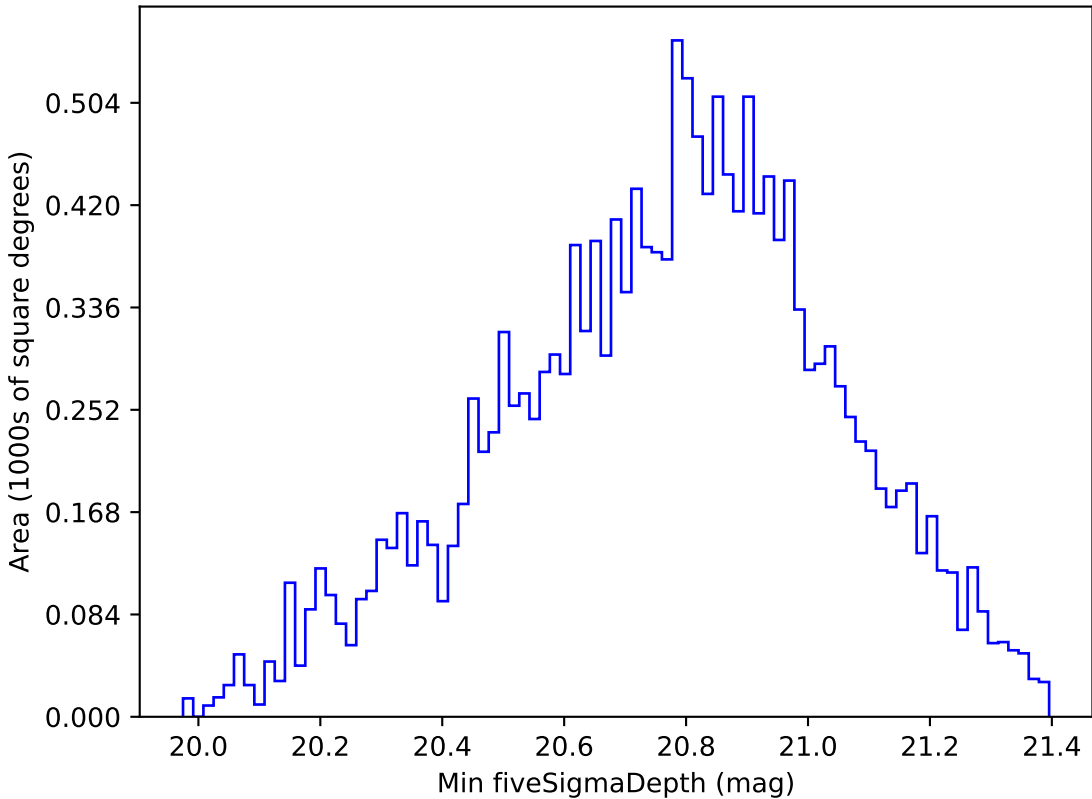
ddf_loaded_fl15_v3.4_10yrs WFD all bands: Min fiveSigmaDepth
