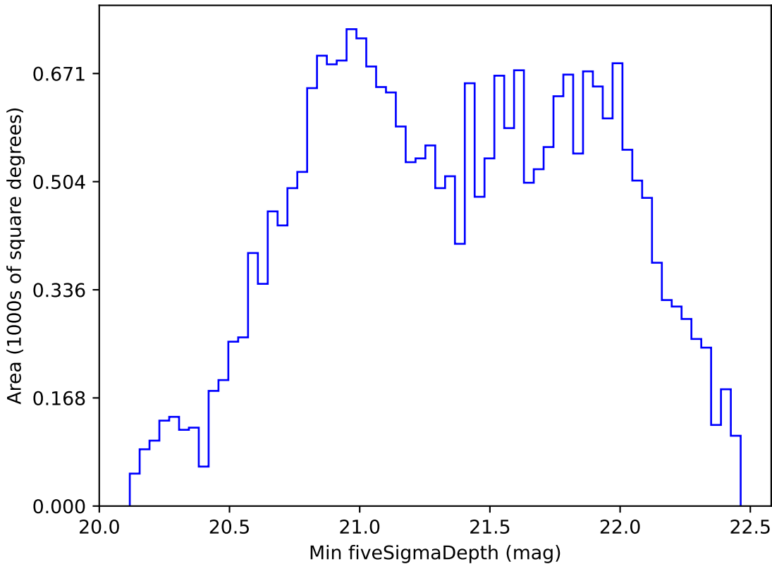
ddf_loaded_fl15_v3.4_10yrs All sky z band: Min fiveSigmaDepth
