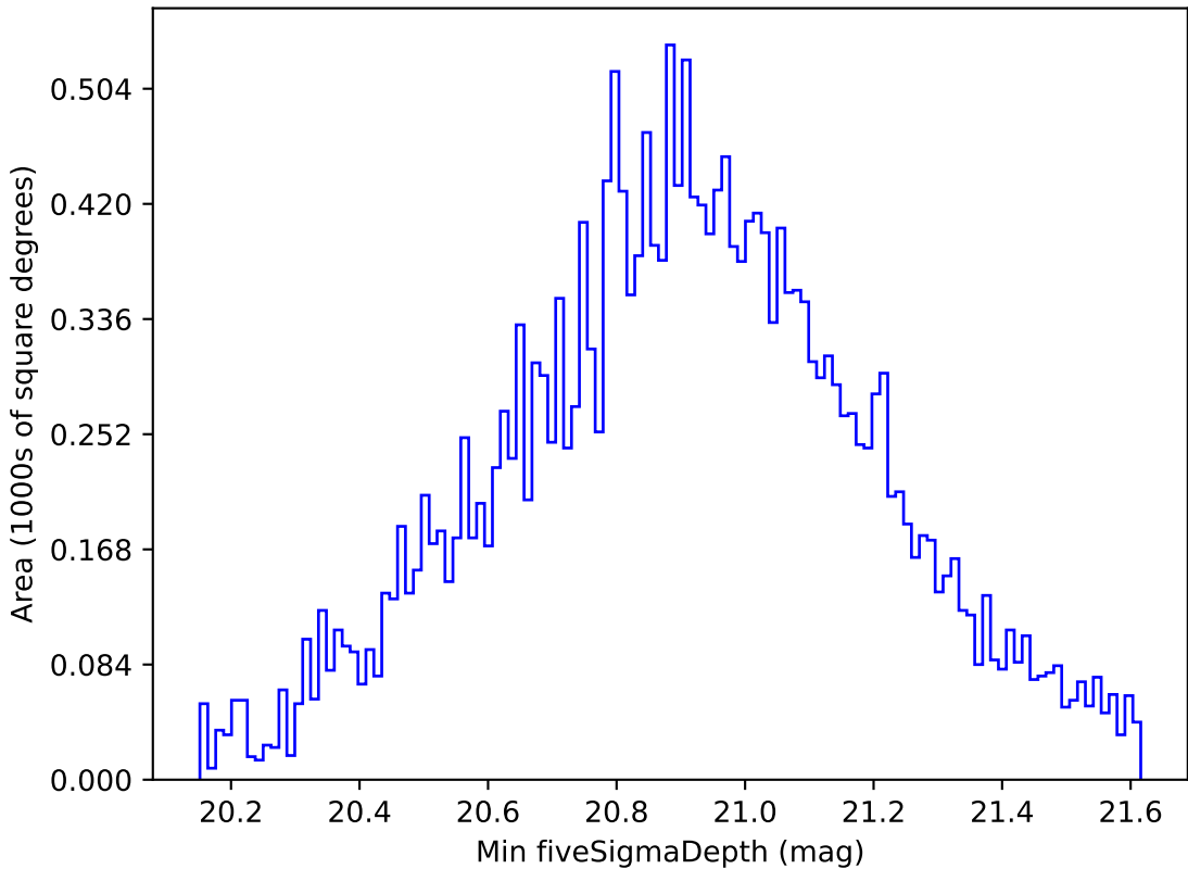
ddf_loaded_fl15_v3.4_10yrs All sky y band: Min fiveSigmaDepth
