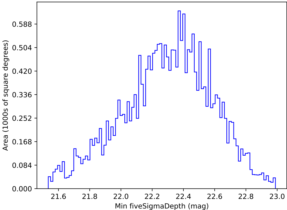
ddf_loaded_fl15_v3.4_10yrs All sky u band: Min fiveSigmaDepth
