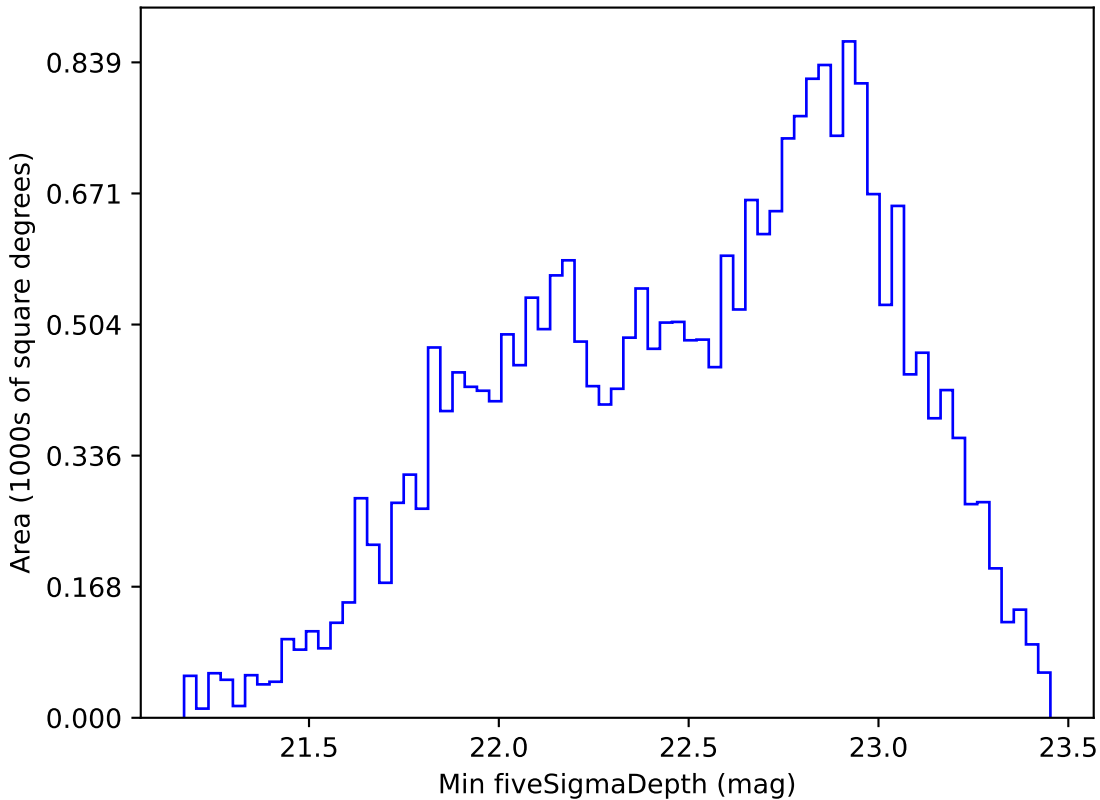
ddf_loaded_fl15_v3.4_10yrs All sky r band: Min fiveSigmaDepth
