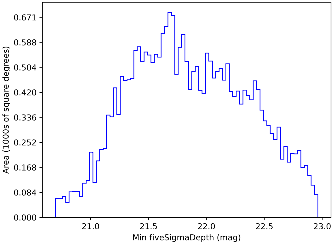
ddf_loaded_fl15_v3.4_10yrs All sky i band: Min fiveSigmaDepth
