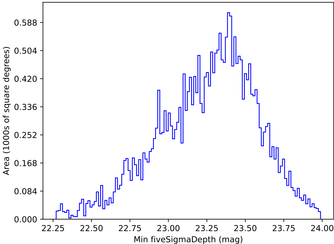
ddf_loaded_fl15_v3.4_10yrs All sky g band: Min fiveSigmaDepth
