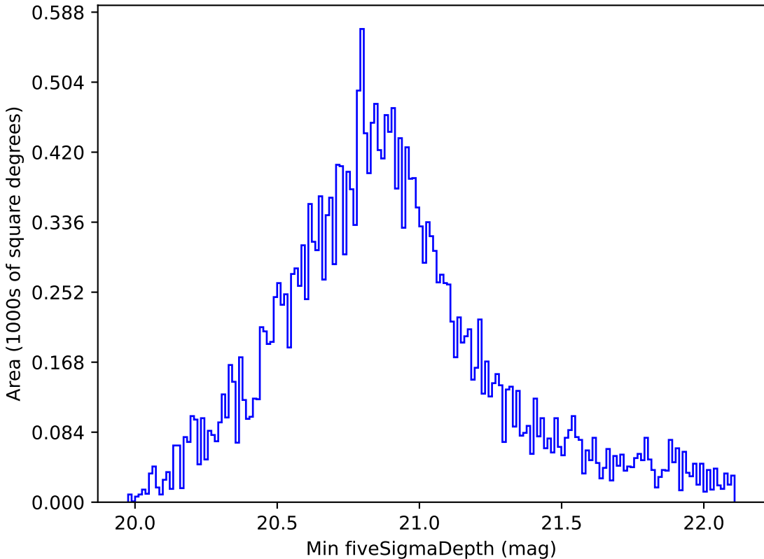
ddf_loaded_fl15_v3.4_10yrs All sky all bands: Min fiveSigmaDepth
