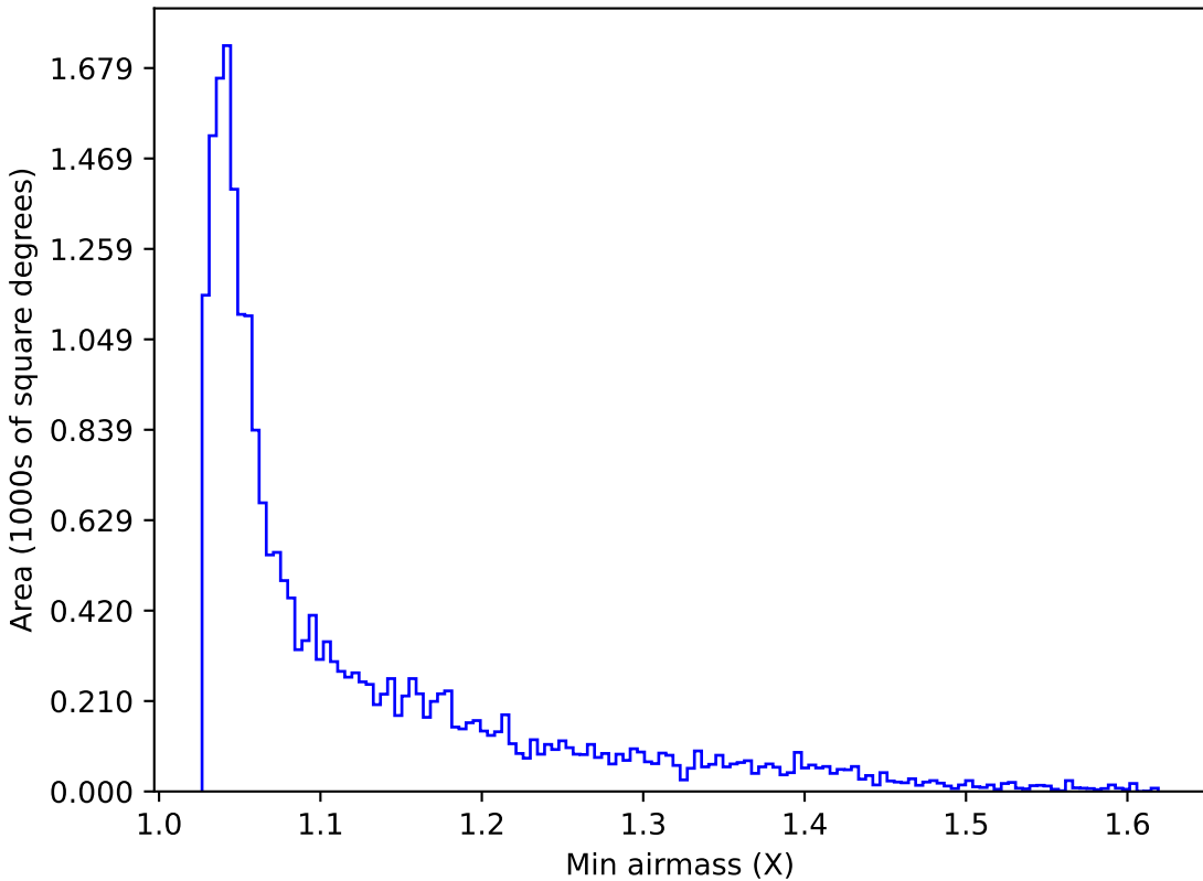
ddf_loaded_fl15_v3.4_10yrs Yr 1 y band: Min airmass
