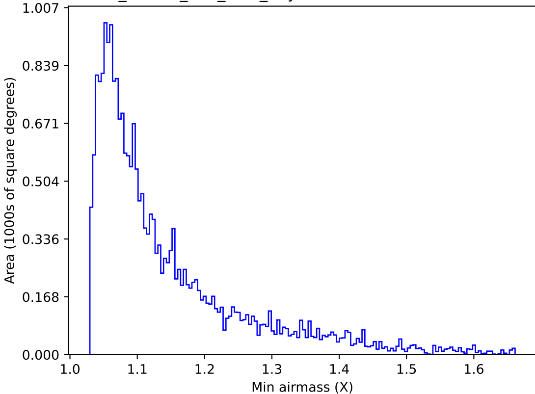
ddf_loaded_fl15_v3.4_10yrs Yr 1 u band: Min airmass
