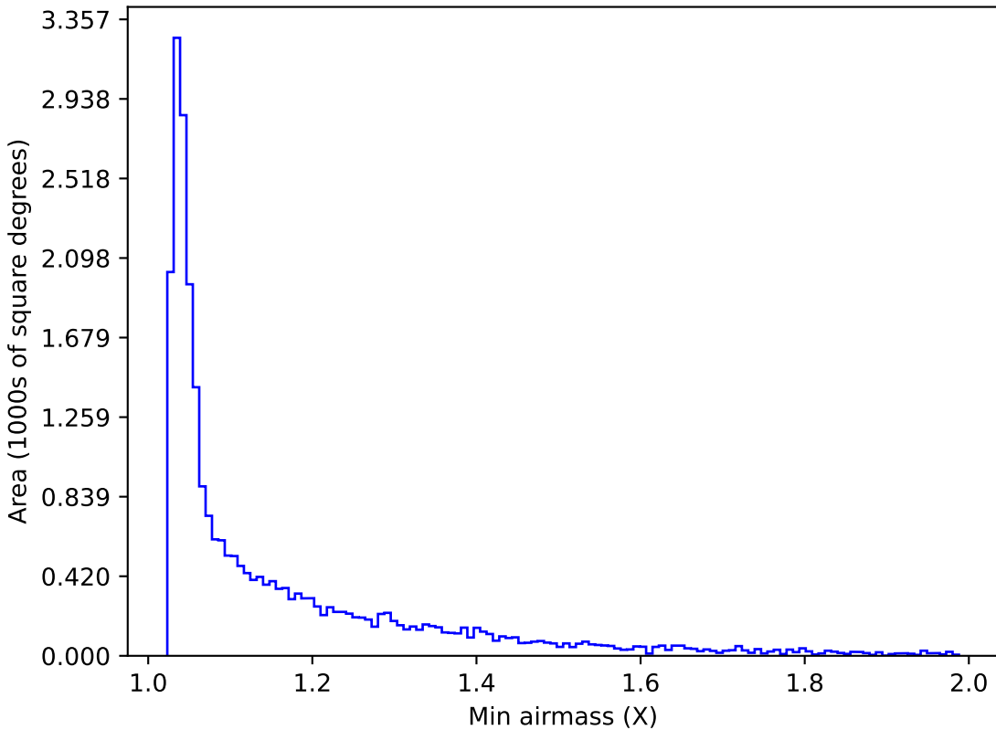
ddf_loaded_fl15_v3.4_10yrs Yr 1 r band: Min airmass
