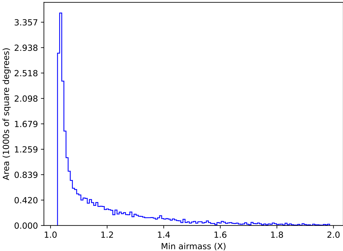
ddf_loaded_fl15_v3.4_10yrs Yr 1 i band: Min airmass
