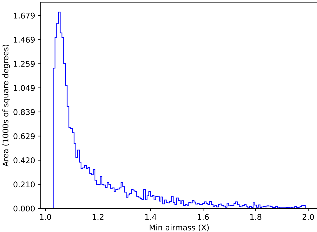
ddf_loaded_fl15_v3.4_10yrs Yr 1 g band: Min airmass
