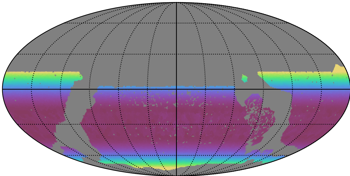
ddf_loaded_fl15_v3.4_10yrs WFD z band: Min airmass
