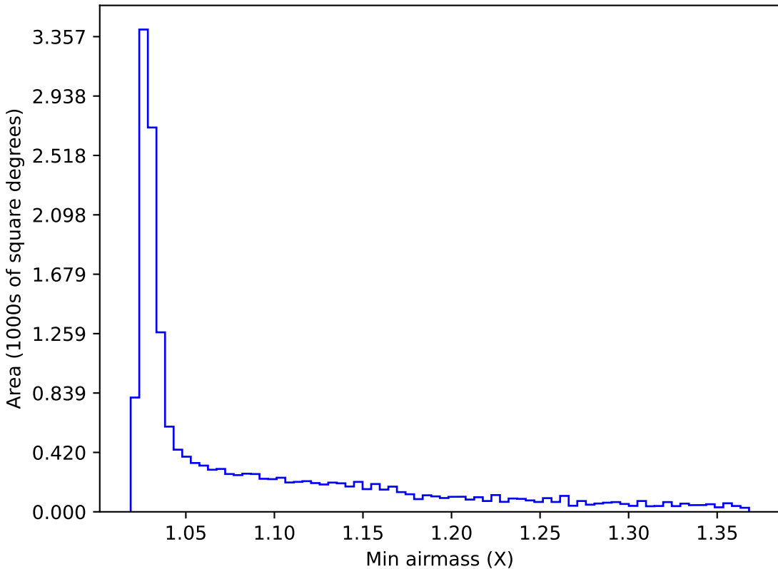
ddf_loaded_fl15_v3.4_10yrs WFD z band: Min airmass
