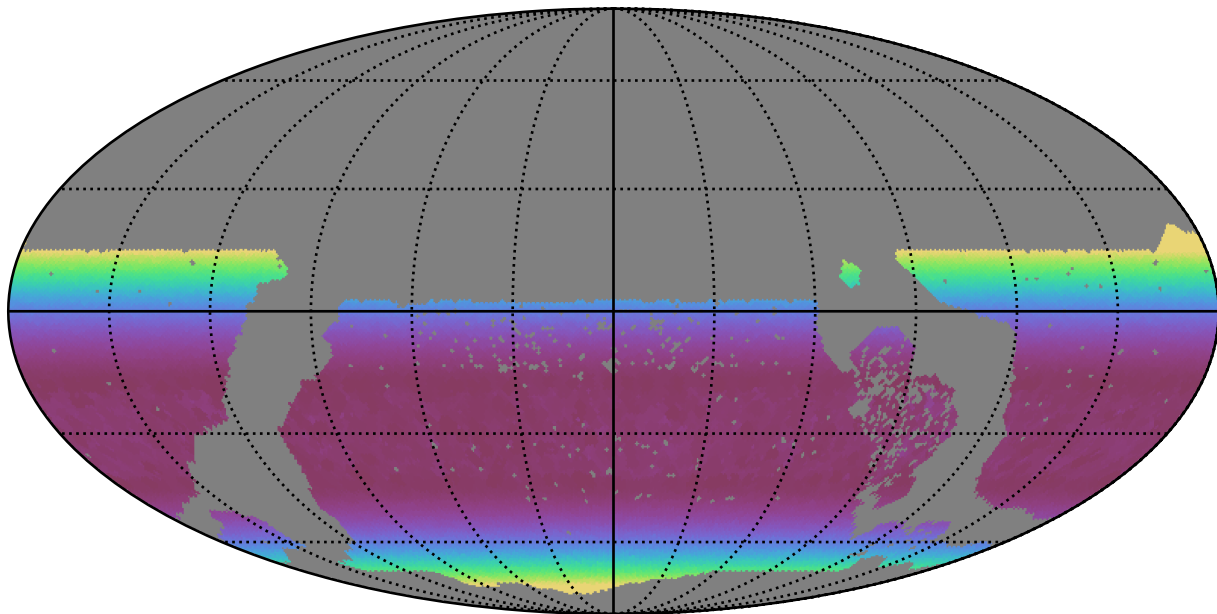
ddf_loaded_fl15_v3.4_10yrs WFD y band: Min airmass
