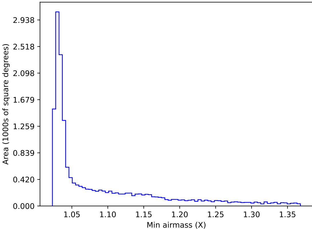
ddf_loaded_fl15_v3.4_10yrs WFD y band: Min airmass
