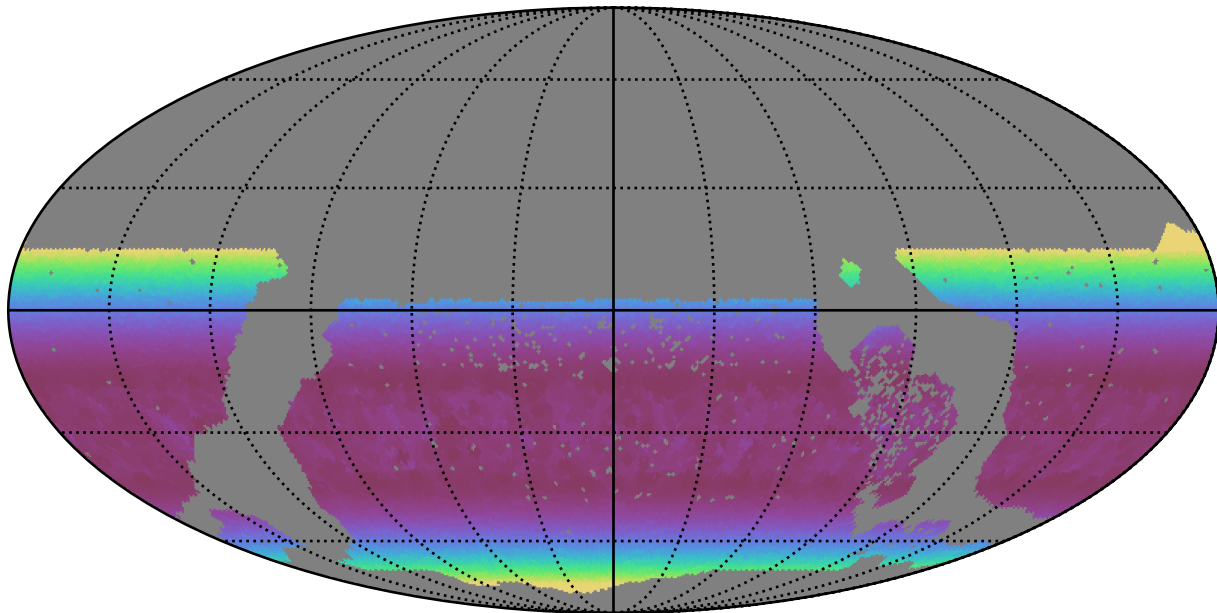
ddf_loaded_fl15_v3.4_10yrs WFD u band: Min airmass
