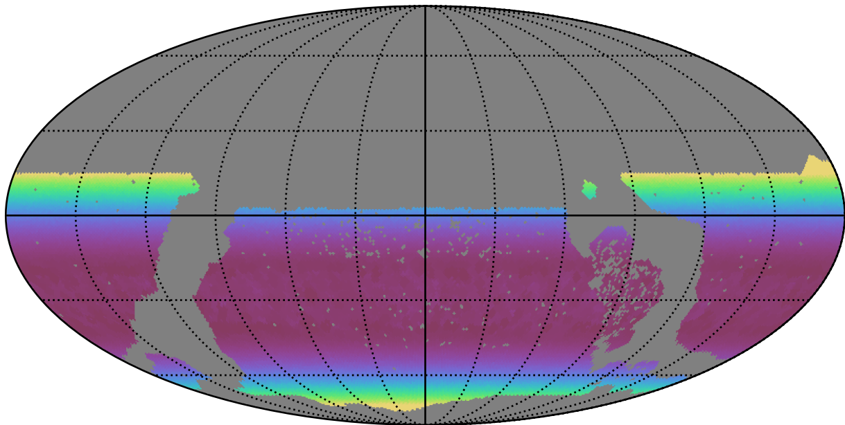
ddf_loaded_fl15_v3.4_10yrs WFD r band: Min airmass
