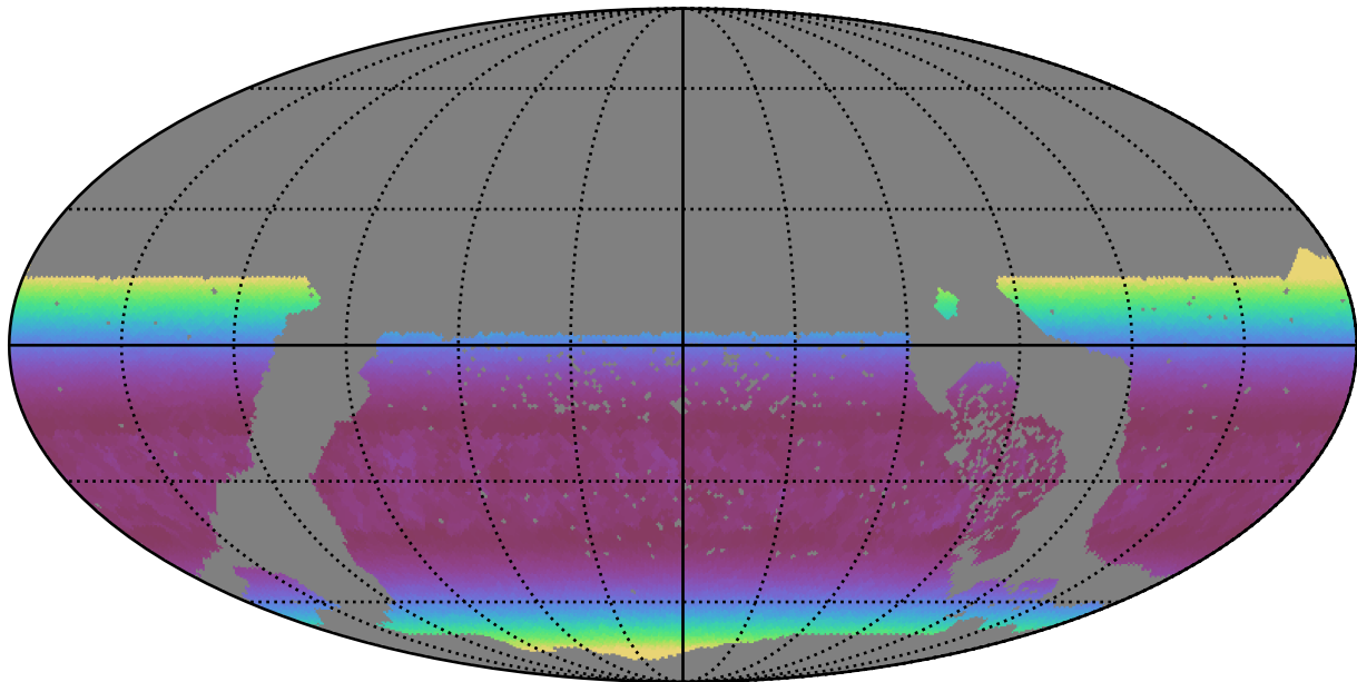
ddf_loaded_fl15_v3.4_10yrs WFD g band: Min airmass
