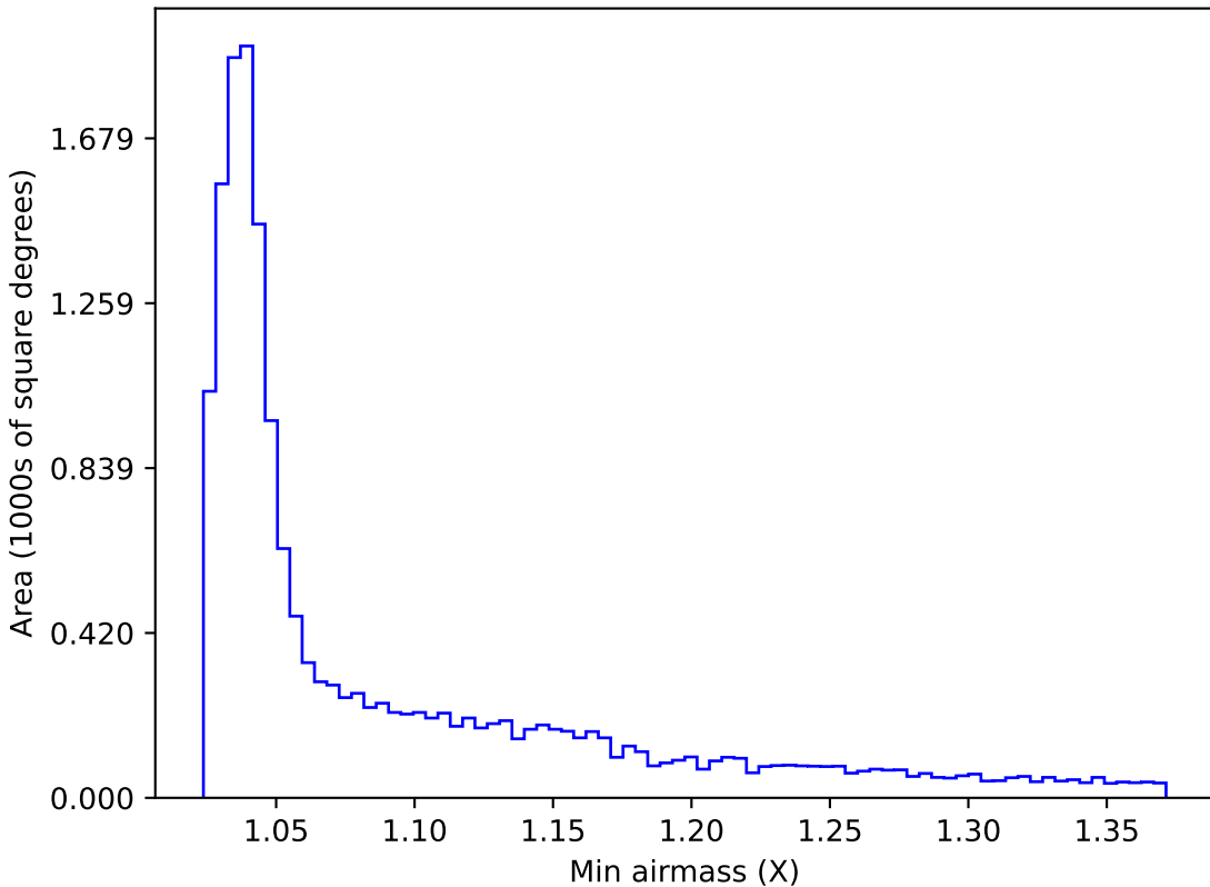
ddf_loaded_fl15_v3.4_10yrs WFD g band: Min airmass
