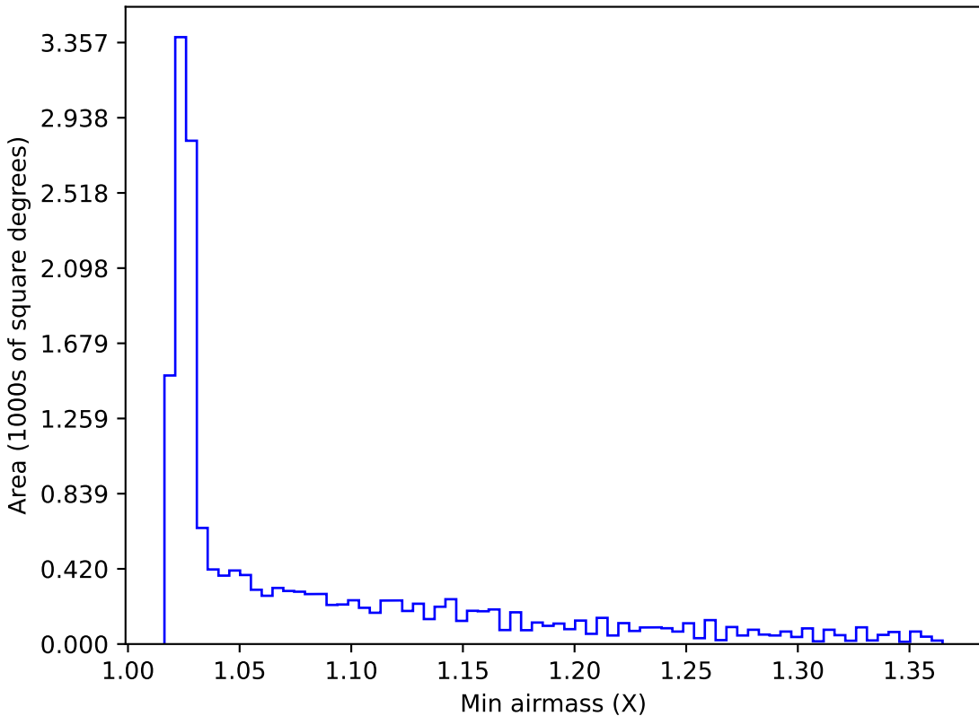
ddf_loaded_fl15_v3.4_10yrs WFD all bands: Min airmass
