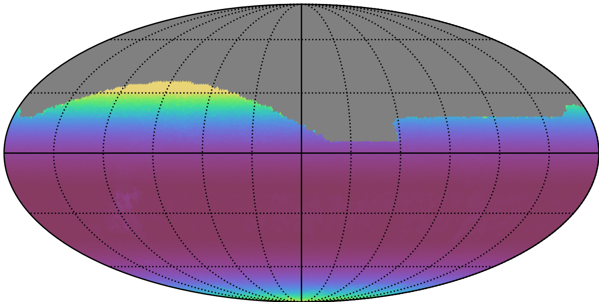
ddf_loaded_fl15_v3.4_10yrs All sky z band: Min airmass
