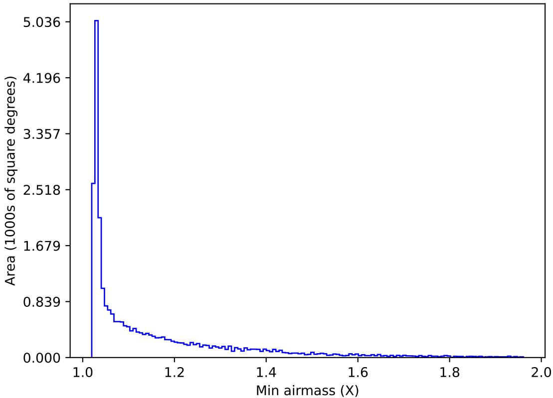
ddf_loaded_fl15_v3.4_10yrs All sky z band: Min airmass
