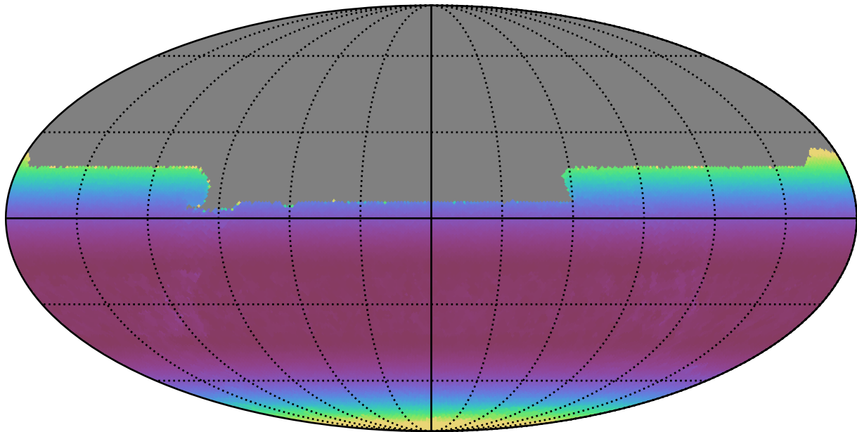
ddf_loaded_fl15_v3.4_10yrs All sky y band: Min airmass
