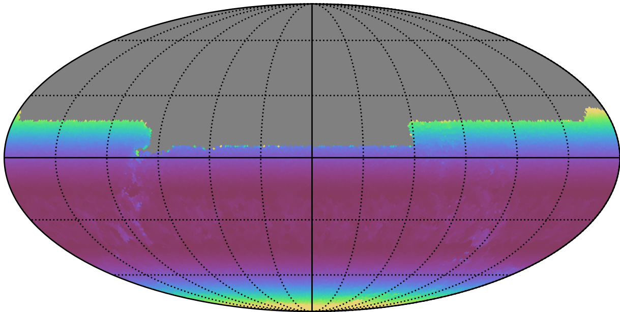
ddf_loaded_fl15_v3.4_10yrs All sky u band: Min airmass
