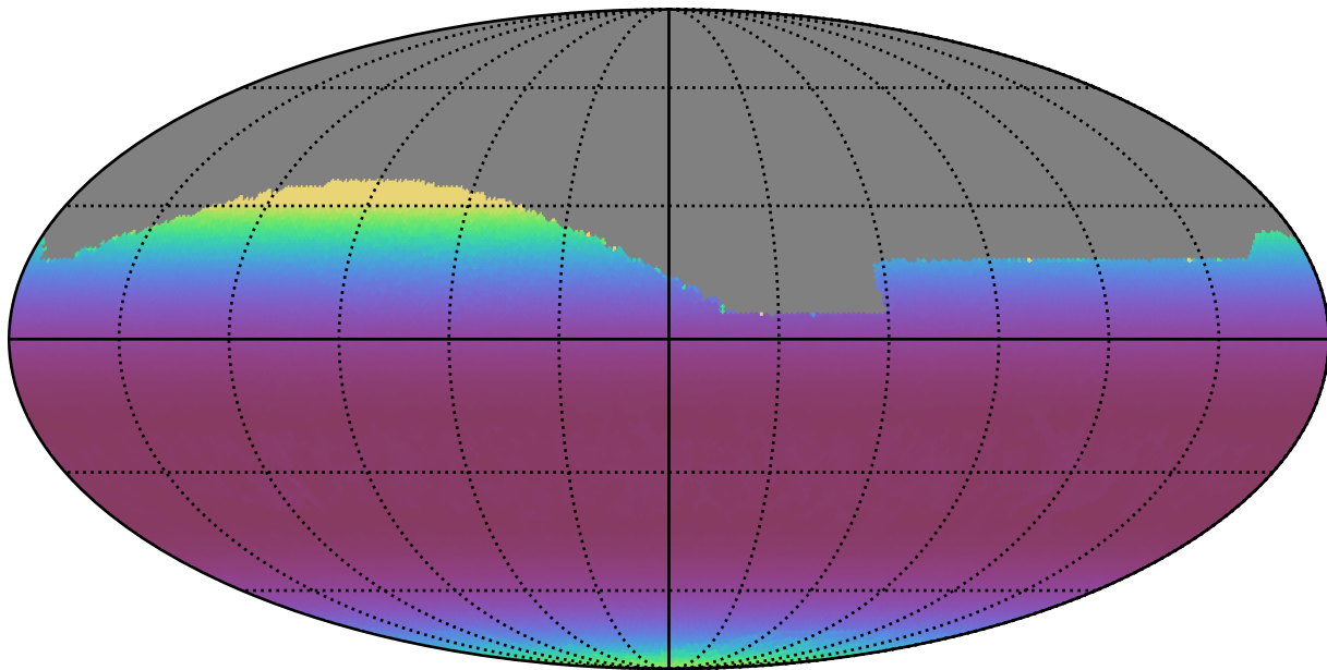
ddf_loaded_fl15_v3.4_10yrs All sky r band: Min airmass
