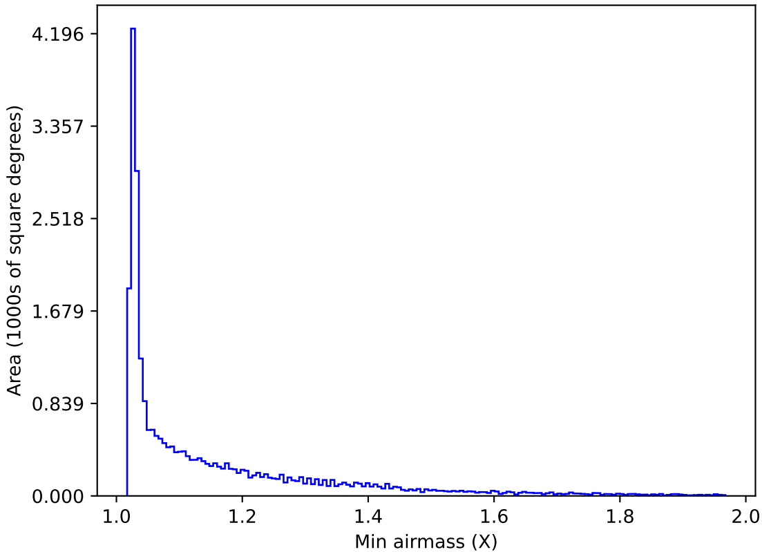
ddf_loaded_fl15_v3.4_10yrs All sky r band: Min airmass
