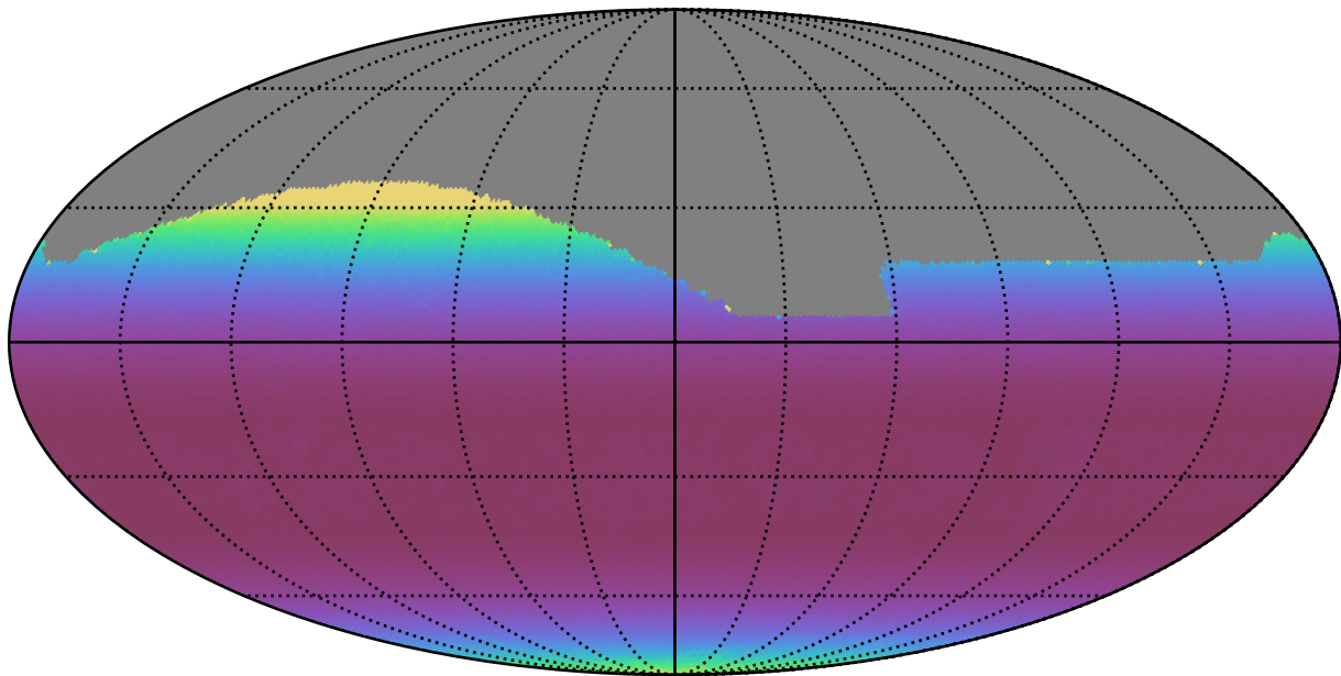
ddf_loaded_fl15_v3.4_10yrs All sky i band: Min airmass
