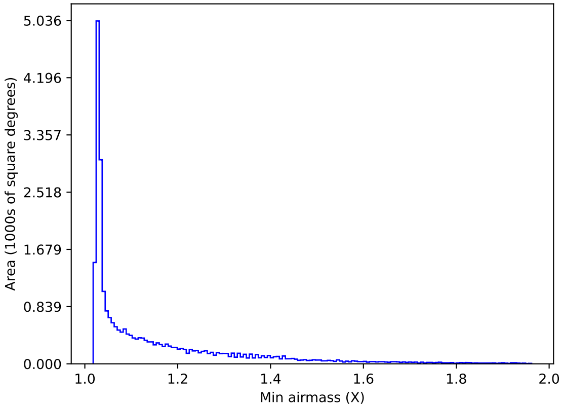
ddf_loaded_fl15_v3.4_10yrs All sky i band: Min airmass
