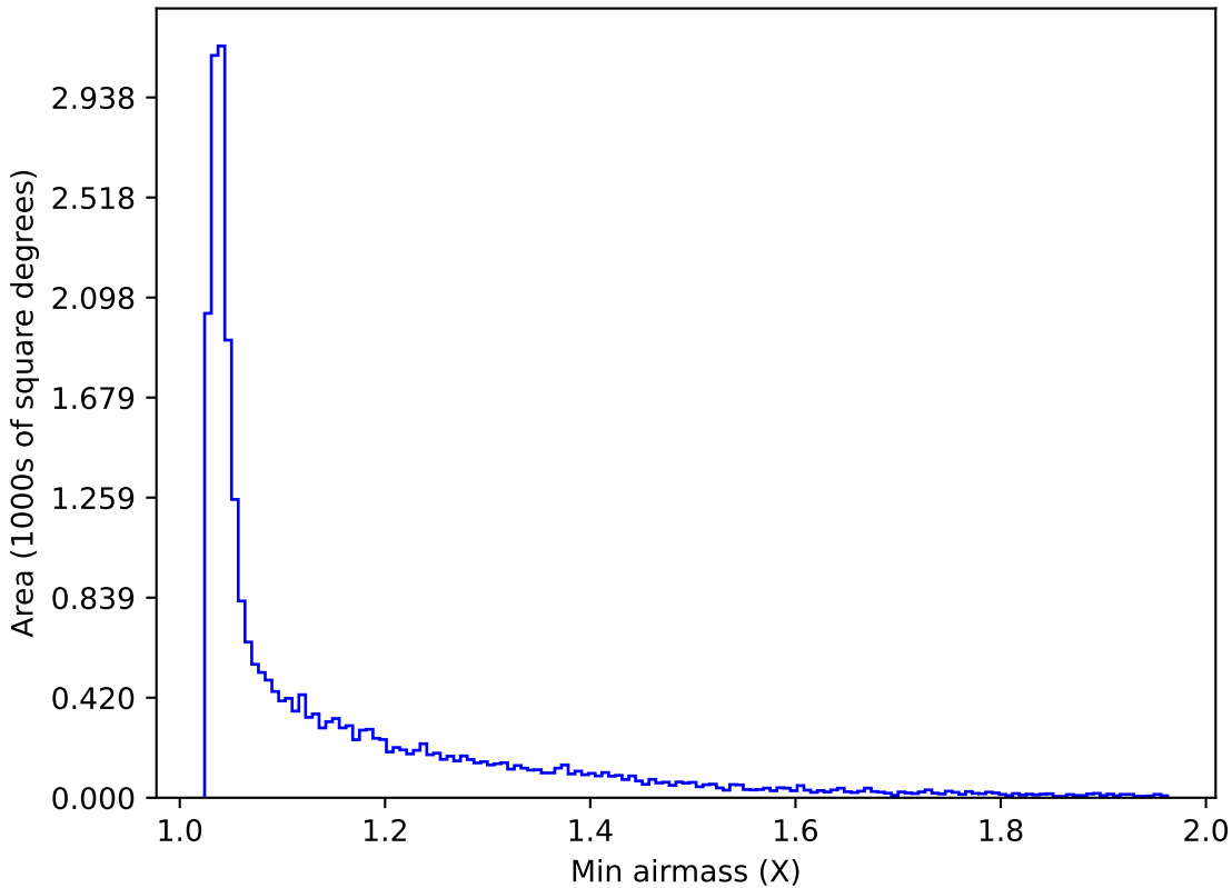
ddf_loaded_fl15_v3.4_10yrs All sky g band: Min airmass
