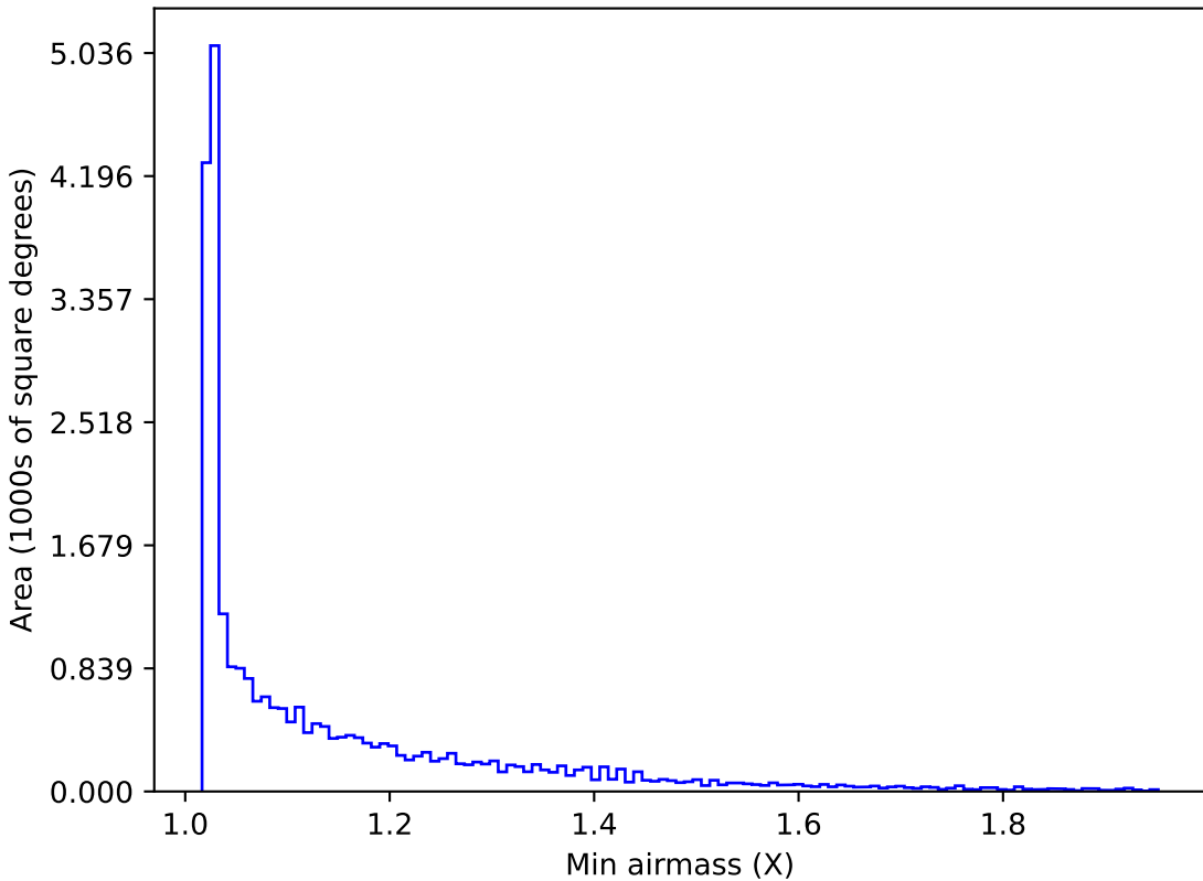
ddf_loaded_fl15_v3.4_10yrs All sky all bands: Min airmass
