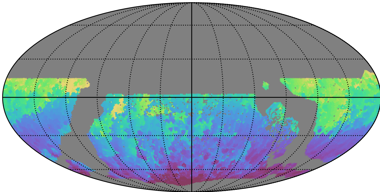
ddf_loaded_fl15_v3.4_10yrs WFD z band: Min HA
