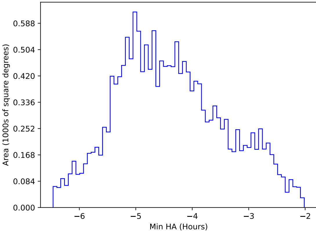
ddf_loaded_fl15_v3.4_10yrs WFD z band: Min HA
