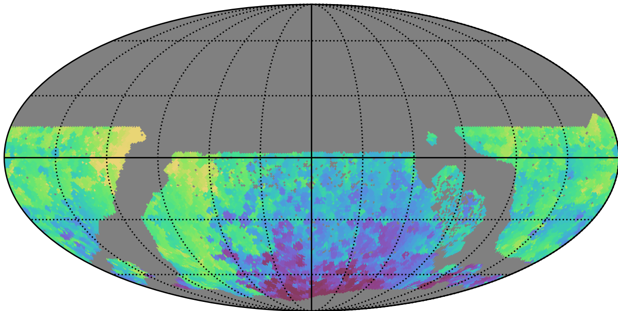
ddf_loaded_fl15_v3.4_10yrs WFD y band: Min HA
