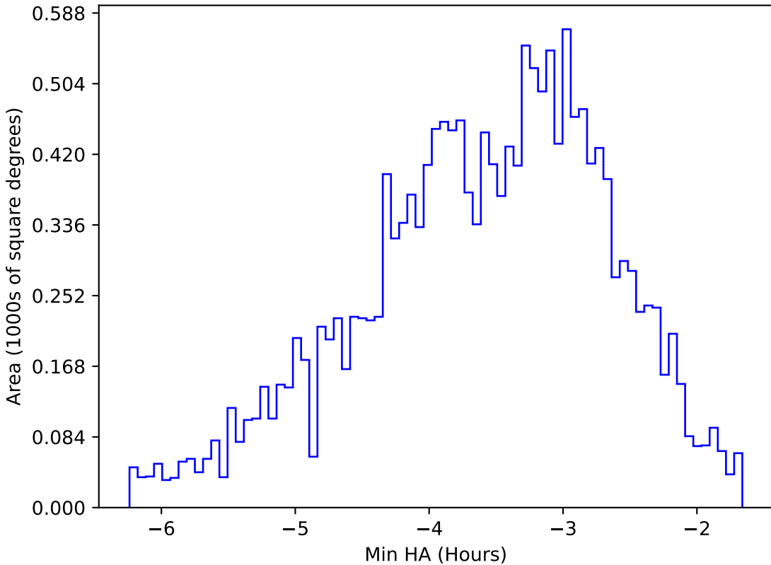
ddf_loaded_fl15_v3.4_10yrs WFD y band: Min HA
