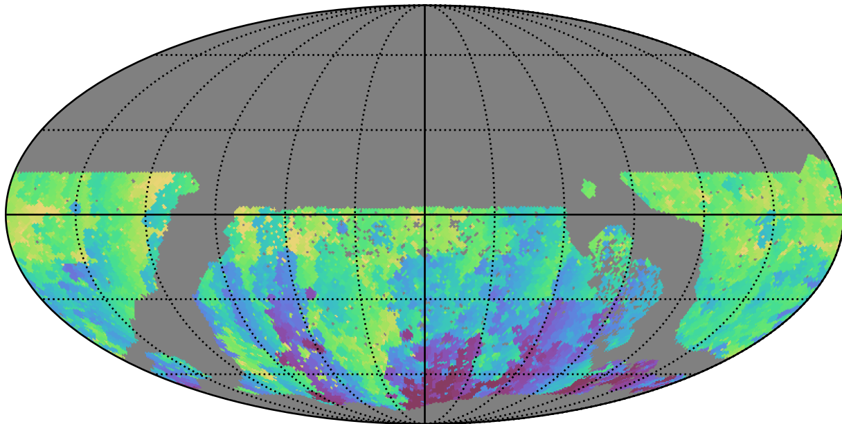
ddf_loaded_fl15_v3.4_10yrs WFD u band: Min HA
