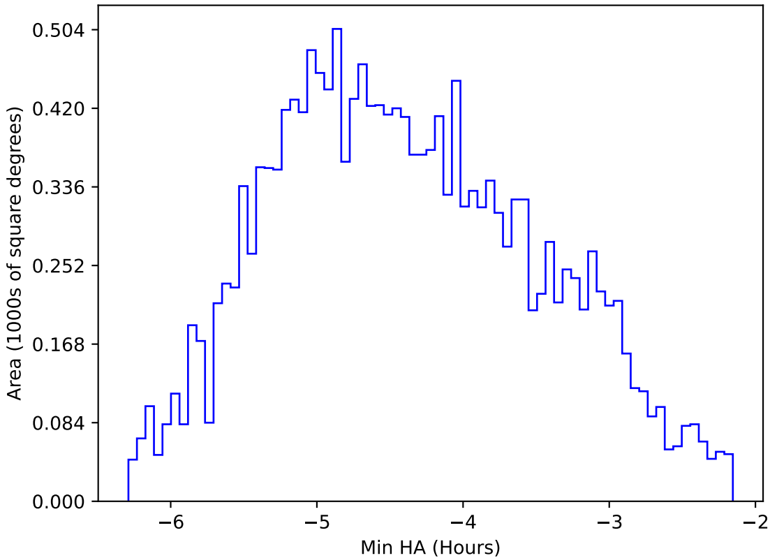
ddf_loaded_fl15_v3.4_10yrs WFD r band: Min HA
