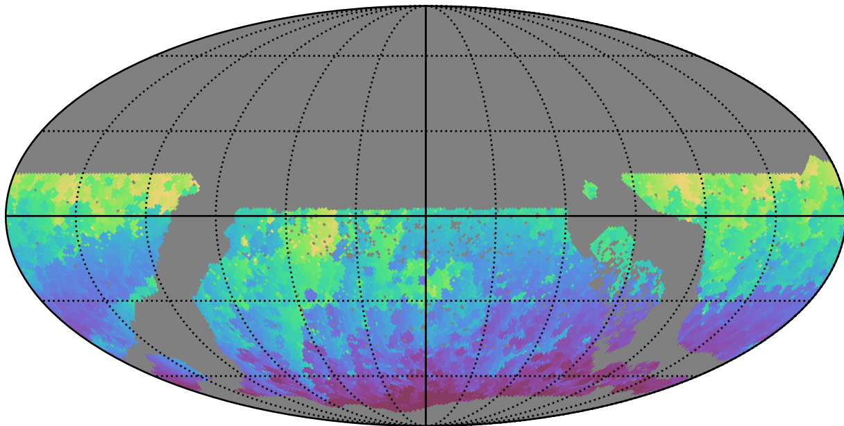
ddf_loaded_fl15_v3.4_10yrs WFD i band: Min HA
