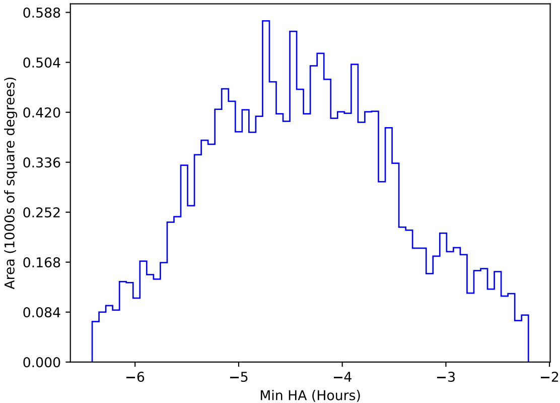
ddf_loaded_fl15_v3.4_10yrs WFD i band: Min HA
