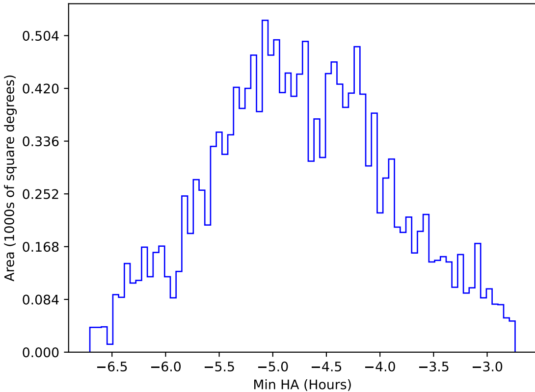
ddf_loaded_fl15_v3.4_10yrs WFD all bands: Min HA
