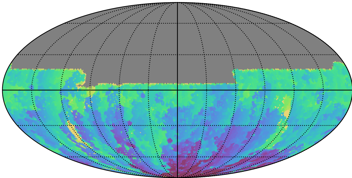
ddf_loaded_fl15_v3.4_10yrs All sky u band: Min HA
