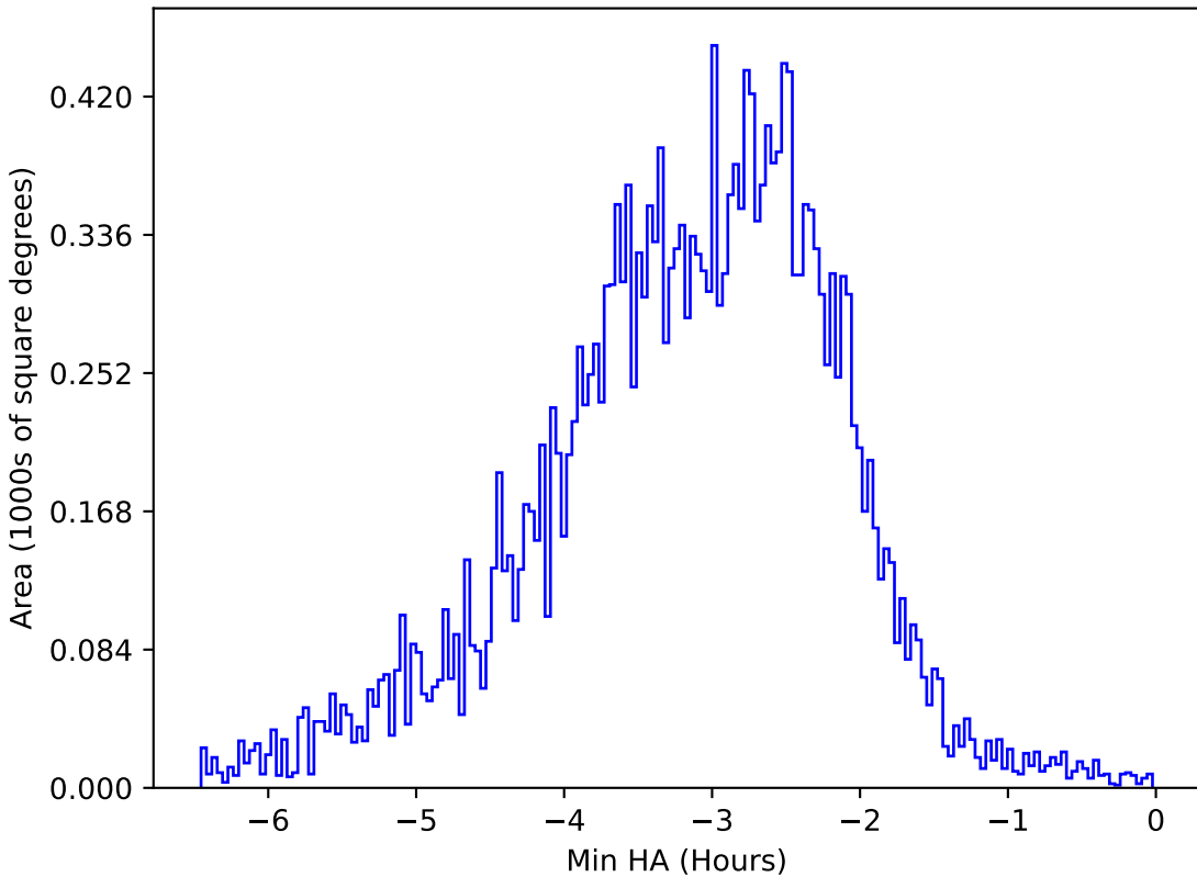
ddf_loaded_fl15_v3.4_10yrs All sky u band: Min HA
