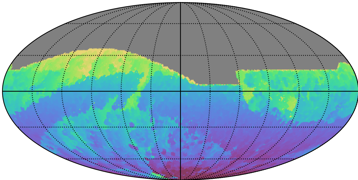
ddf_loaded_fl15_v3.4_10yrs All sky r band: Min HA
