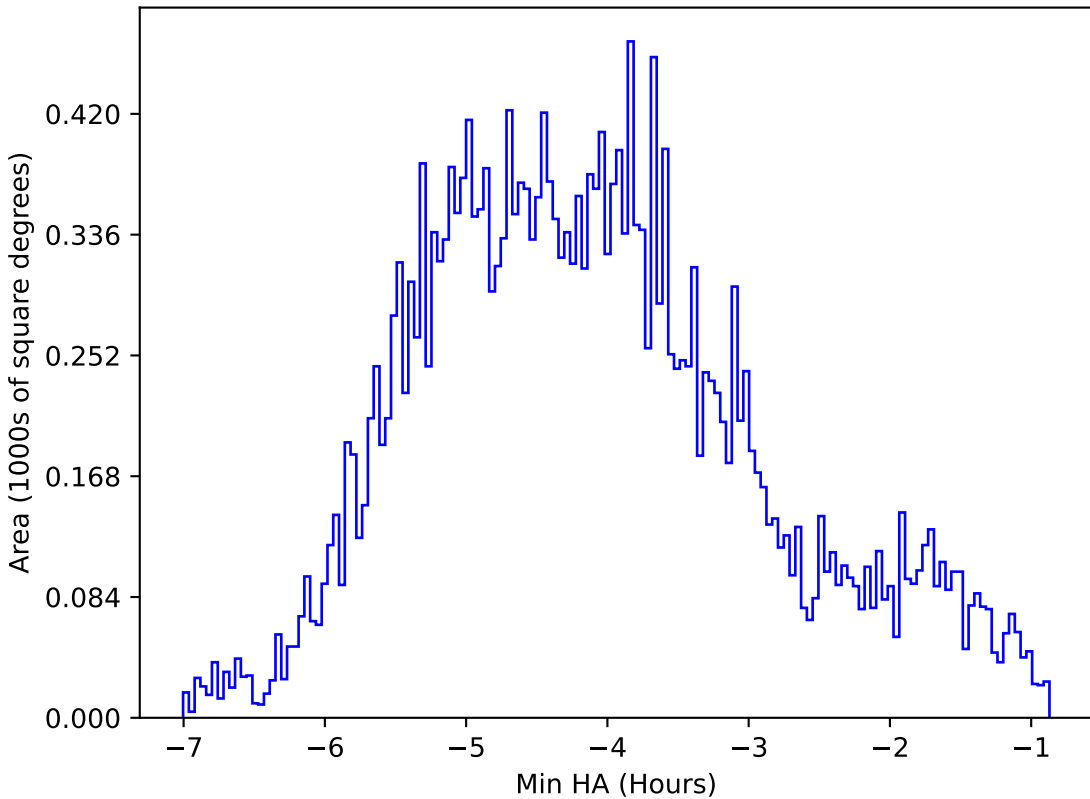
ddf_loaded_fl15_v3.4_10yrs All sky r band: Min HA
