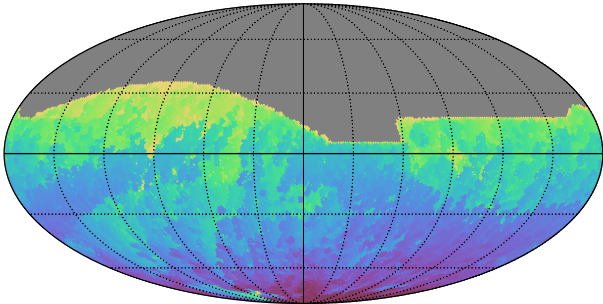
ddf_loaded_fl15_v3.4_10yrs All sky i band: Min HA
