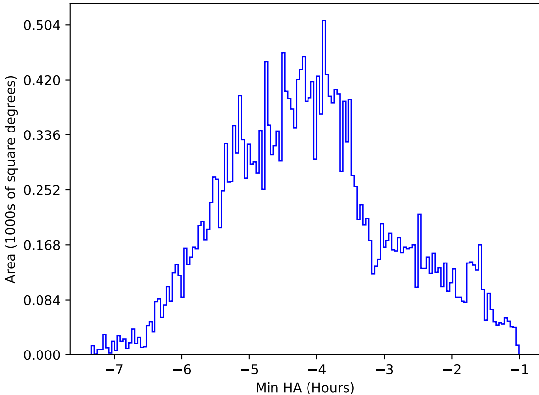
ddf_loaded_fl15_v3.4_10yrs All sky i band: Min HA
