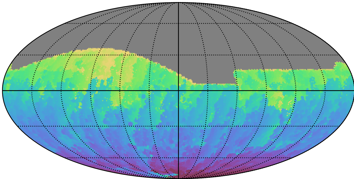
ddf_loaded_fl15_v3.4_10yrs All sky g band: Min HA
