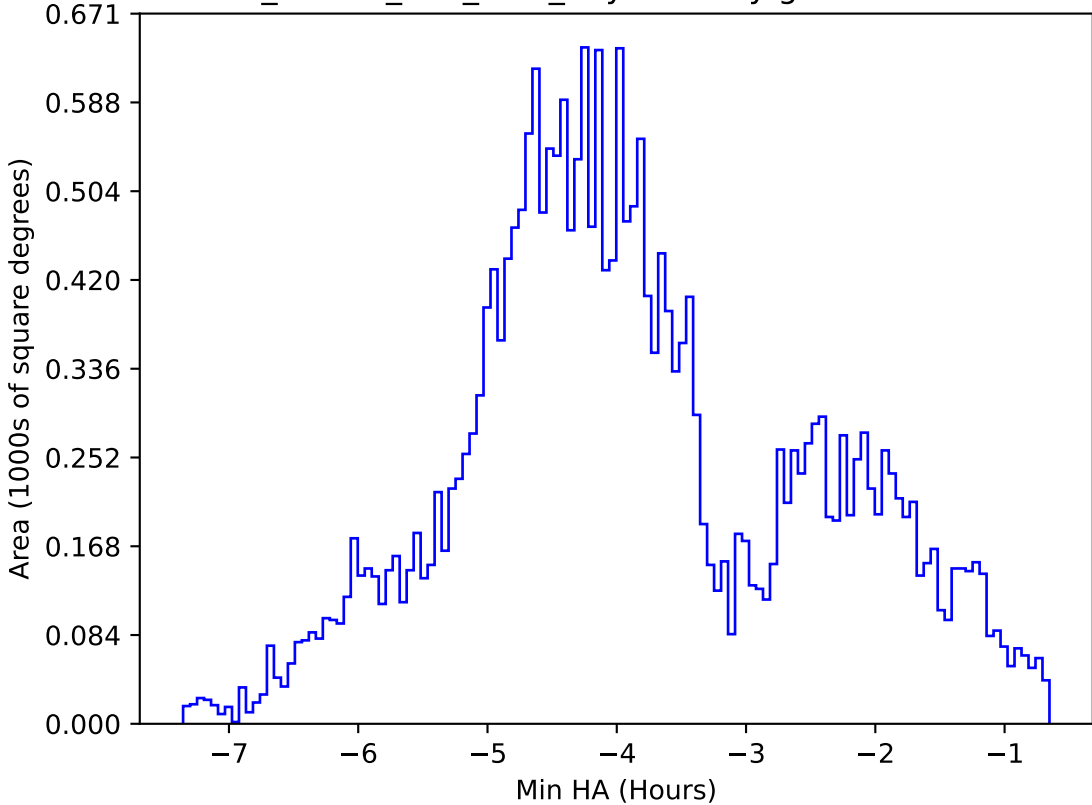
ddf_loaded_fl15_v3.4_10yrs All sky g band: Min HA
